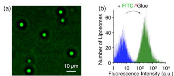
Figure 3. Adhesion of fluorescently labeled molecular glue FITC- 9 Glue onto a phospholipid membrane in HEPES buffer (10 mM HEPES, 100 mM NaCl, pH 7.0). (a) Fluorescence microscopy ( \lambda_{\text{ext}} = 488 nm) of giant EYPC liposomes (140 μM) containing FITC- 9 Glue (25 nM). (b) Flow cytometry histograms ( \lambda_{\text{ext}} = 488 nm) of giant EYPC liposomes (140 μM) before (blue) and after (green) mixing with FITC- 9 Glue (25 nM).
