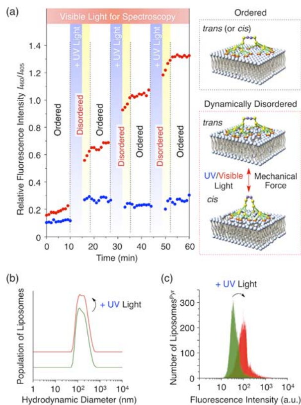
Figure 4. Transmembrane ion permeation profiles of pyranine-containing EYPC liposomes (35 \mu\text{M} ; initial inner pH = 7.0) at 25 ^{\circ}\text{C} in HEPES buffer (10 mM HEPES, 100 mM NaCl, pH 8.4) containing Azo- 18 Glue (1.5 \mu\text{M} ) or Azo- 6 Glue (4.5 \mu\text{M} ) ( [\text{Gu}^+] = 27 \mu\text{M} ). (a) Changes in relative fluorescence intensity I_{460}/I_{405} at 510 nm ( \lambda_{\text{ext}} = 460 and 405 nm for I_{460} and I_{405} , respectively) upon on-off photoirradiation of Azo- 18 Glue (red circles) and Azo- 6 Glue (blue circles) with a 365-nm external UV light (blue-shaded areas). Enhanced I_{460}/I_{405} is the consequence of an increment of the inner pH by \text{OH}^- permeation, possibly by photomechanically induced disordering of the liposomal membrane (Figure 2b). Note that the sample in yellow-shaded areas was exposed to visible excitation lights for fluorescence spectroscopy, so that cis -Azo- 18 Glue likely isomerized back to its trans -form. This isomerization may also give rise to disordering of the liposomal membrane (Figure 2b). (b) DLS histograms of EYPC liposomes before (green) and after (red) 15 min photoirradiation of Azo- 18 Glue with a 365-nm UV light. (c) Flow cytometry histograms ( \lambda_{\text{ext}} = 488 \text{ nm} ) of pyranine-containing giant EYPC liposomes before (green) and after (red) 10-min photoirradiation of Azo- 18 Glue with a 365-nm UV light.
