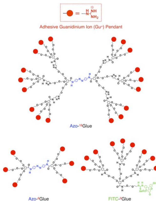
Figure 1. Schematic structures of photoresponsive molecular glues Azo- 6 Glue and Azo- 18 Glue together with that of fluorescently labeled molecular glue FITC- 9 Glue. Red circles represent adhesive guanidinium ion (Gu + ) pendants.
