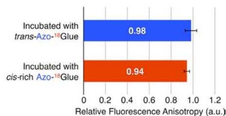
Figure 5. Static adhesion effects of Azo- 18 Glue on the fluidity of a phospholipid membrane. Fluorescence depolarization profiles at 25 ^{\circ}\text{C} of DPH (70 nM), embedded in an Azo- 18 Glue-attached EYPC liposomal membrane (35 \mu\text{M} ), relative to that without Azo- 18 Glue, in HEPES buffer (10 mM HEPES, 100 mM NaCl, pH 7.0) containing 1.5 \mu\text{M} trans - (blue bar) or cis -rich 12 Azo- 18 Glue (red bar).
