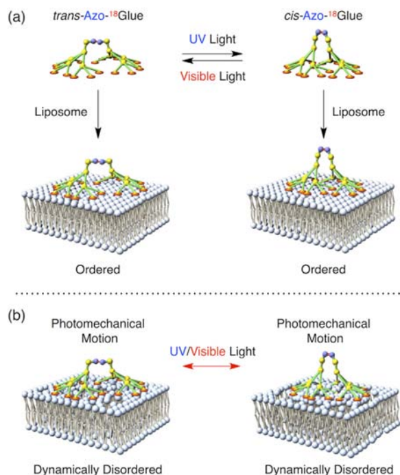
Figure 2. Schematic representations of possible effects of photo-responsive molecular glue Azo- 18 Glue on a phospholipid membrane. (a) Static adhesion effects of trans -Azo- 18 Glue (left) and cis -Azo- 18 Glue (right). In either case, structural disorder is unlikely for the phospholipid membrane due to a thermodynamic equilibration. (b) Dynamic effects of trans -to- cis (left) and cis -to- trans (right) photoisomerization events of adhering Azo- 18 Glue. In either case, a dynamic structural disorder, allowing for transmembrane ion permeation (see Figure 4a), can be expected for the phospholipid membrane by an abrupt photomechanical motion of Azo- 18 Glue.
